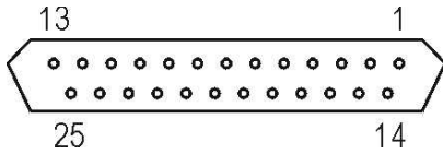
Alarm Switch Pin Assignment Table
